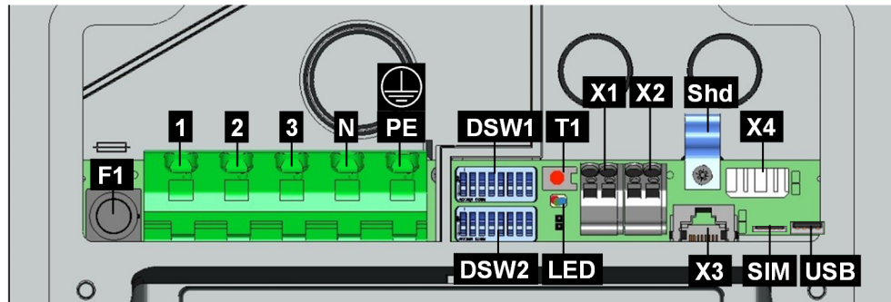
Fig. 7-15: Connection overview
